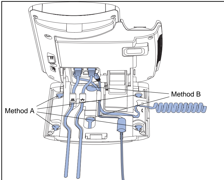
Figure 10: Cable routing tracks and mounting holes
